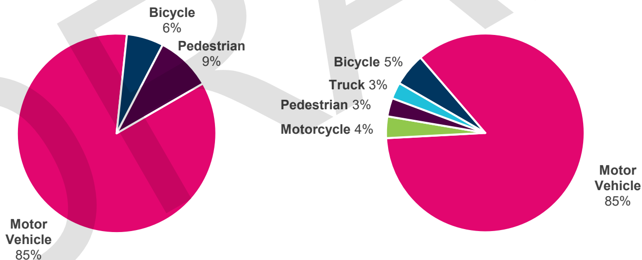
Figure 4. OVERALL TRIPS (LEFT) AND OVERALL CRASHES (RIGHT) BY TRAVEL MODE (ICBC, 2017-2021)
