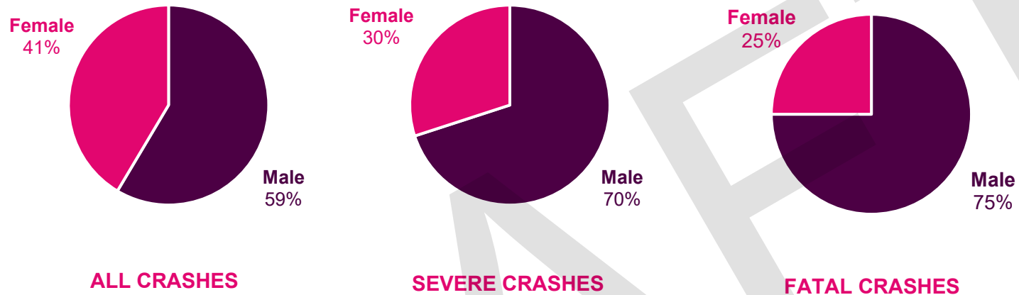
Figure 21. CRASH TRENDS BY GENDER (TAS, 2016-2020)
