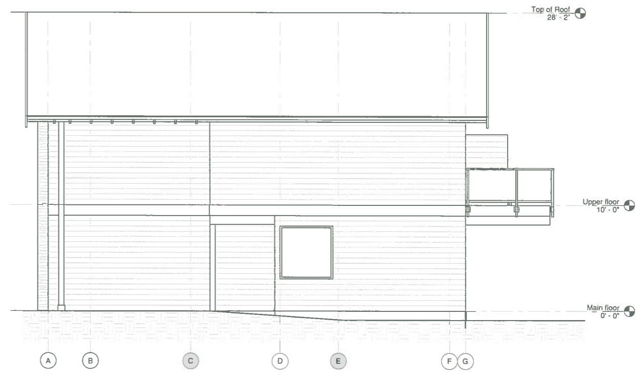
RIGHT SIDE ELEVATION (NORTH) 1/4" = 1'-0"
