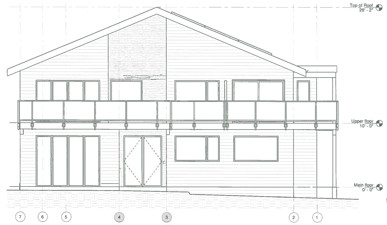
REAR ELEVATION (WEST) 1/4" = 1'-0"
