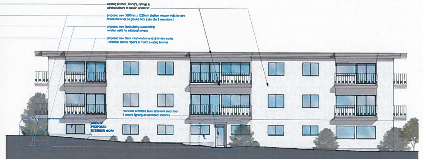
Proposed Rear Elevation [South] metric scale 1 : 100
