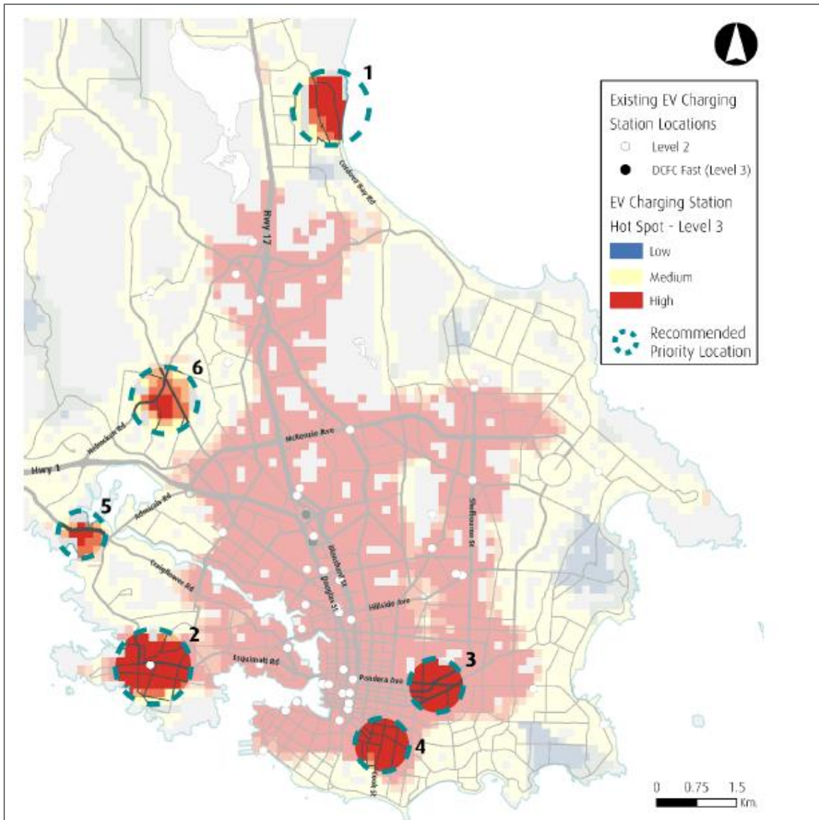
Figure 16: Recommended Priority Locations for Level 2 Charging Stations, Core Area
