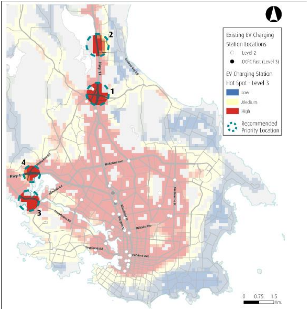
Figure 17: Recommended Priority Locations for Level 3 Charging Stations, Core Area
