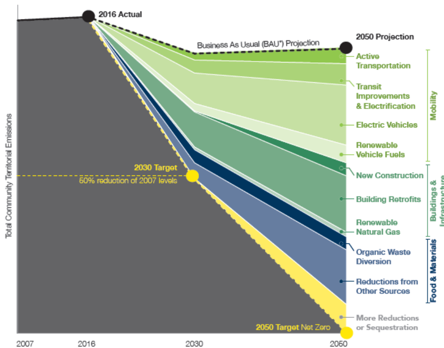
Figure 4: Modeled pathway to reach net-zero GHG emissions in Saanich by 2050
