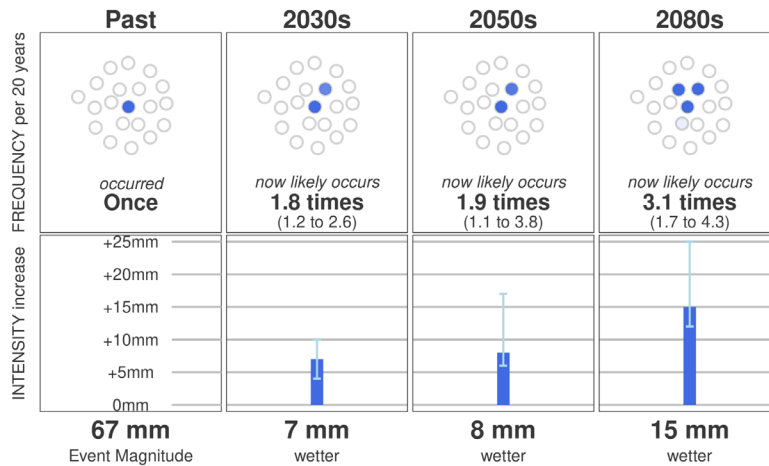
Figure 4. Projected changes in 20 Year Event 1 Day Extreme Rain in CRD Core Municipalities. 8
