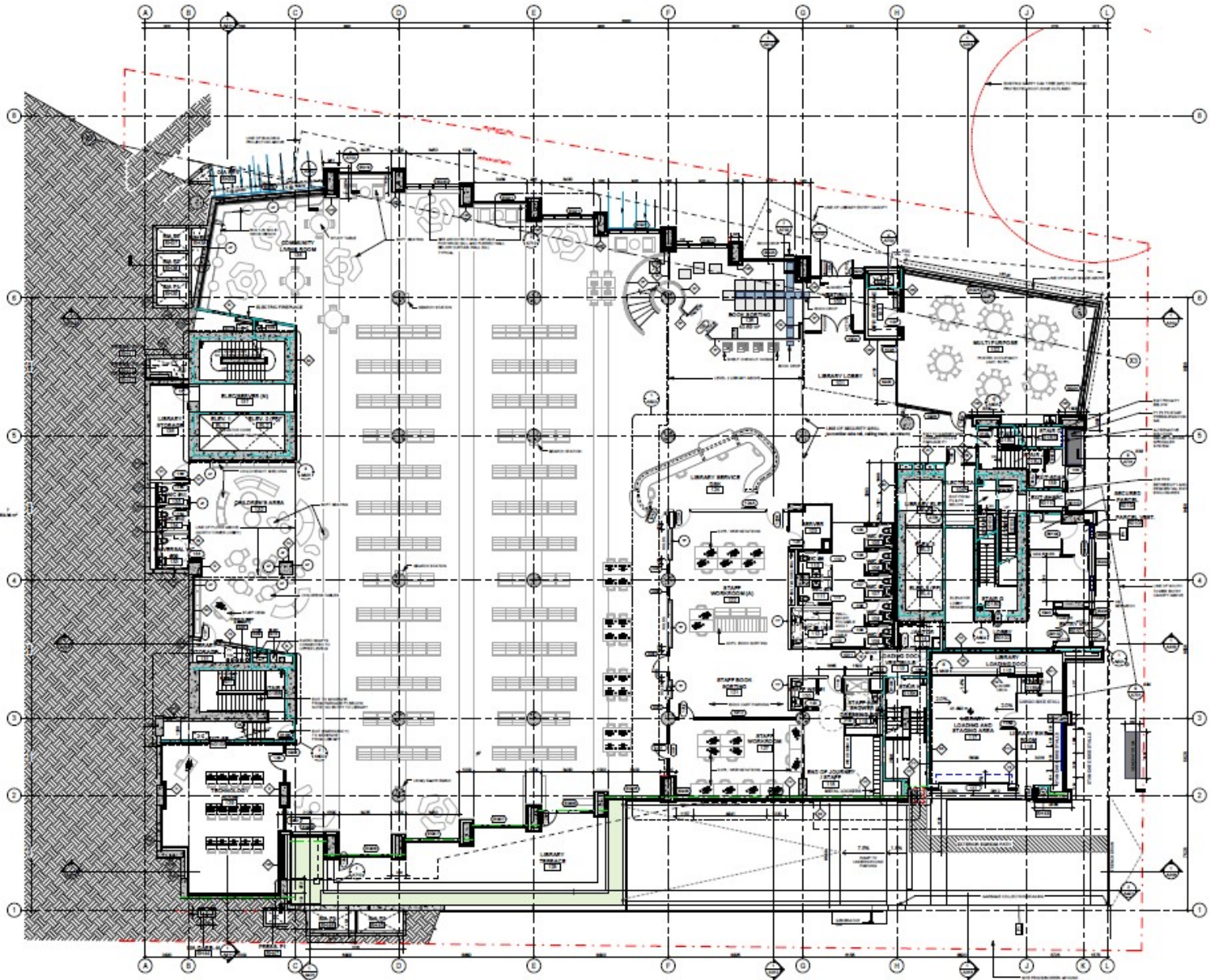
1 FLOOR PLAN - PODIUM LEVEL 01 1/8" = 1'-0"
