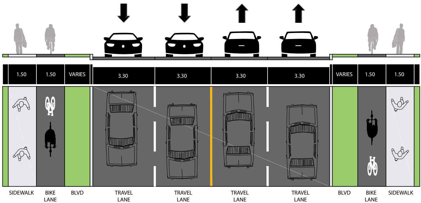
Figure 6.6 | Typical Short-term/ Existing Shelbourne Street Cross-Section (Case 1: Pear Street to Christmas Avenue)
