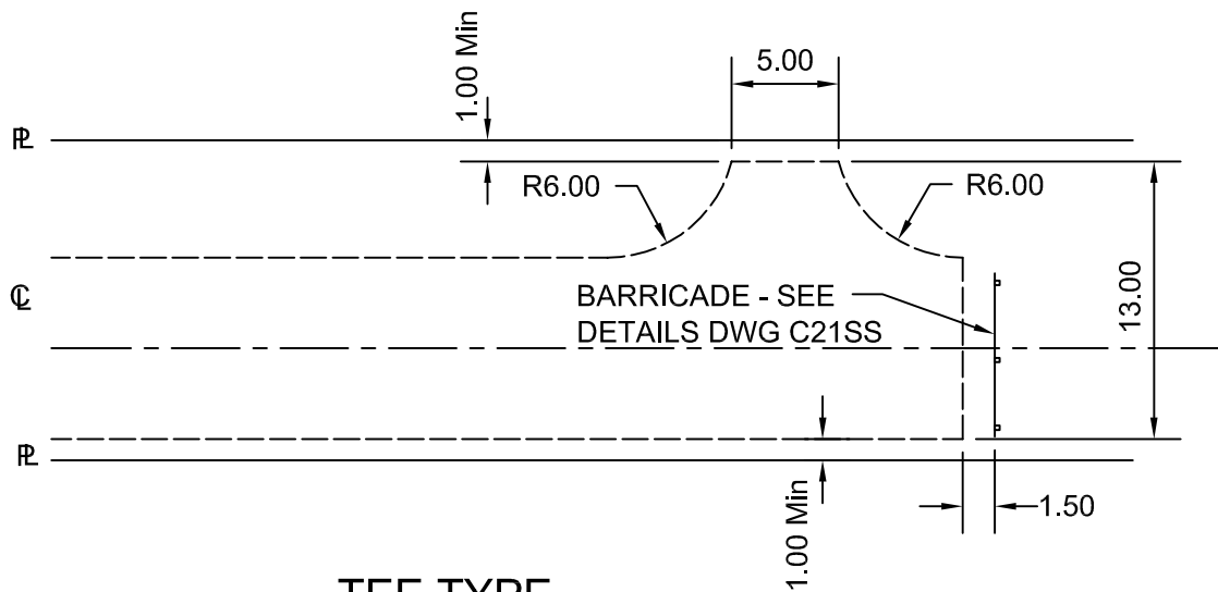
TEE TYPE (FOR OFFSET PAVEMENT)
