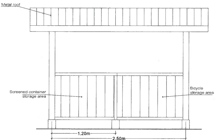
Waste containers and bicycles shelter detail
