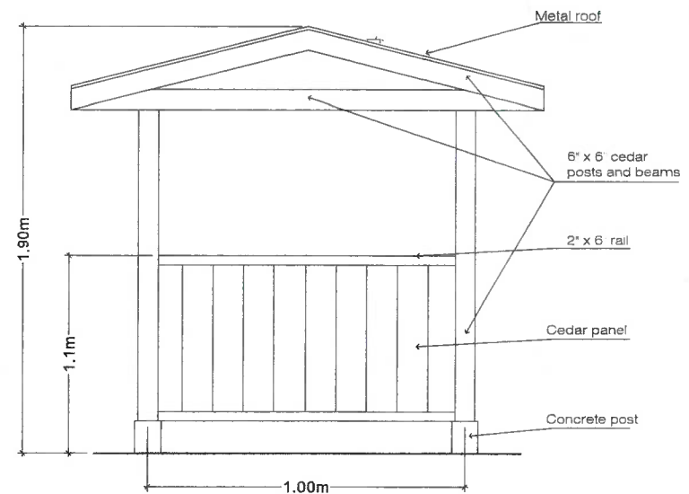
Waste containers and bicycles shelter detail
